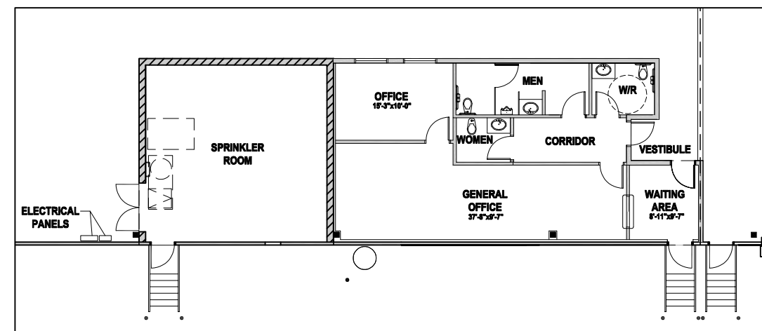
SHIPPING OFFICE SCALE: 1/8"=1'-0" WHEN PRINTED ON 24"x36" SHEET SCALE: FEET
